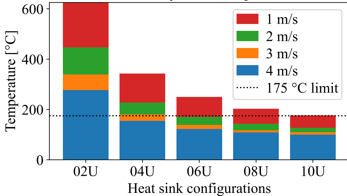
Maximum junction temperature
